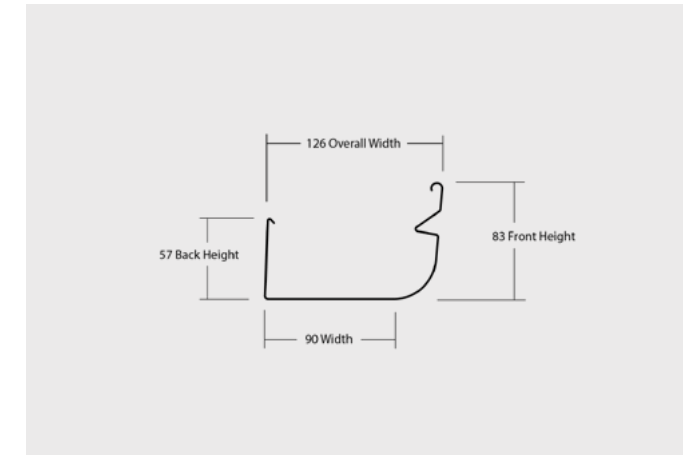
INFINITLINE GUTTER
