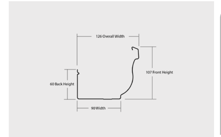
TRAD-LINE™ GUTTER
