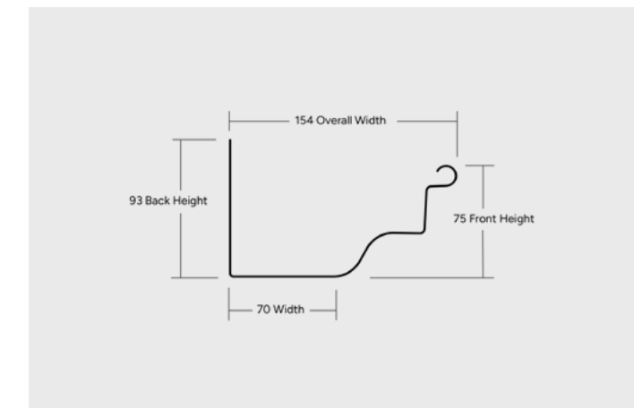
HERITAGE O-GEE 125 GUTTER (NSW)
