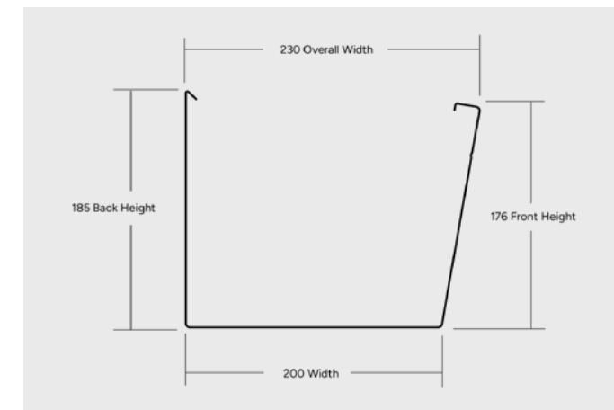
COMMERCIAL EAVES GUTTER (QLD)
