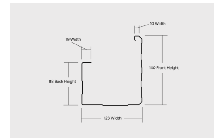
FASCIA GUTTER (VIC)
