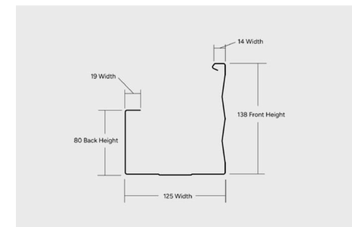
TRILINE SIFFENED BACK (NSW)
