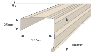
Stramit® Fascia Capping
