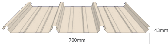
Stramit Speed Deck Ultra®
