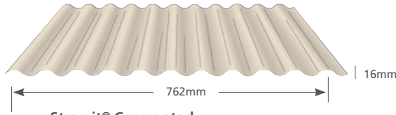
Stramit® Corrugated (also available in Bullnosing and Curving)
