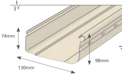
Stramit Queenslander Quad® Slotted Hi-Front
