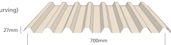
Stramit Longspan®
