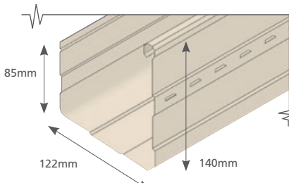
Stramit® M-Pattern Gutter Slotted
