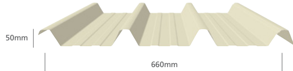
Stramit CapacityPLUS™ 660
